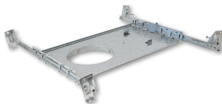
NFC-R430 for 4" only NQZ-6R-F for 6" only NFC-R725 for 8" only Frame-In with Collar
